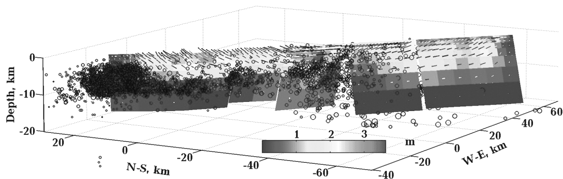
Fig. 1. Coseismic slip model of the El Mayor earthquake derived from inversion of InSAR and GPS Figure data. Colors denote the slip magnitude and arrows denote the sense of slip on the west side of the fault. Black circles denote precisely relocated hypocenters of aftershocks from the time period of 2 months following the mainshock (courtesy of Egill Hauksson).
